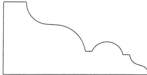
TE794 Solid Crown 1 3/8" x 2 3/4"
